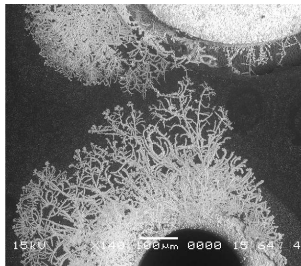
Figure 3. HDD with ImAg surface finish. Cu_2S precipitates out of solution in a dendritic structure.
