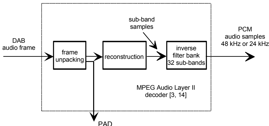
Figure 2122: Simplified block diagram of the DAB audio decoder
