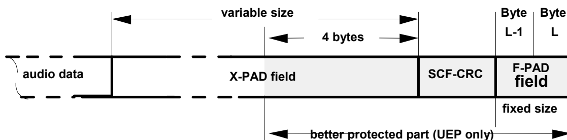
Figure 2627: Location of the PAD bytes within the DAB audio frame
