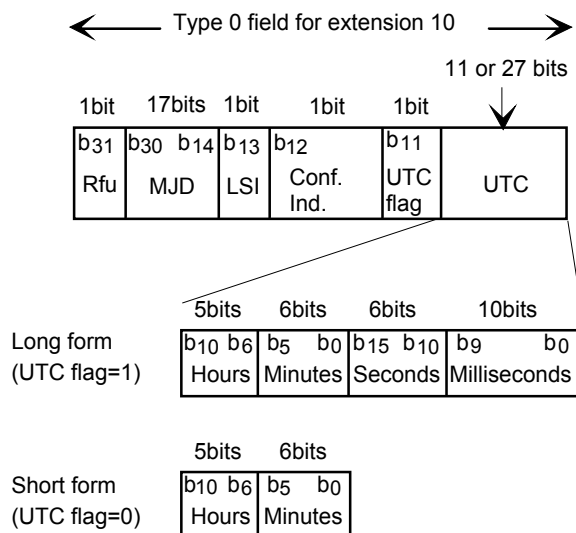
Figure 3537: Structure of the date and time field
