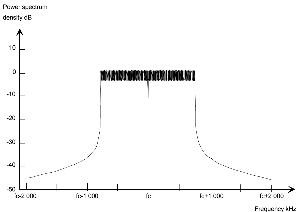
Figure 86409: Theoretical DAB transmission signal spectrum for transmission mode IV
