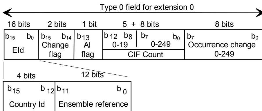
Figure 1920: Structure of the ensemble information field
