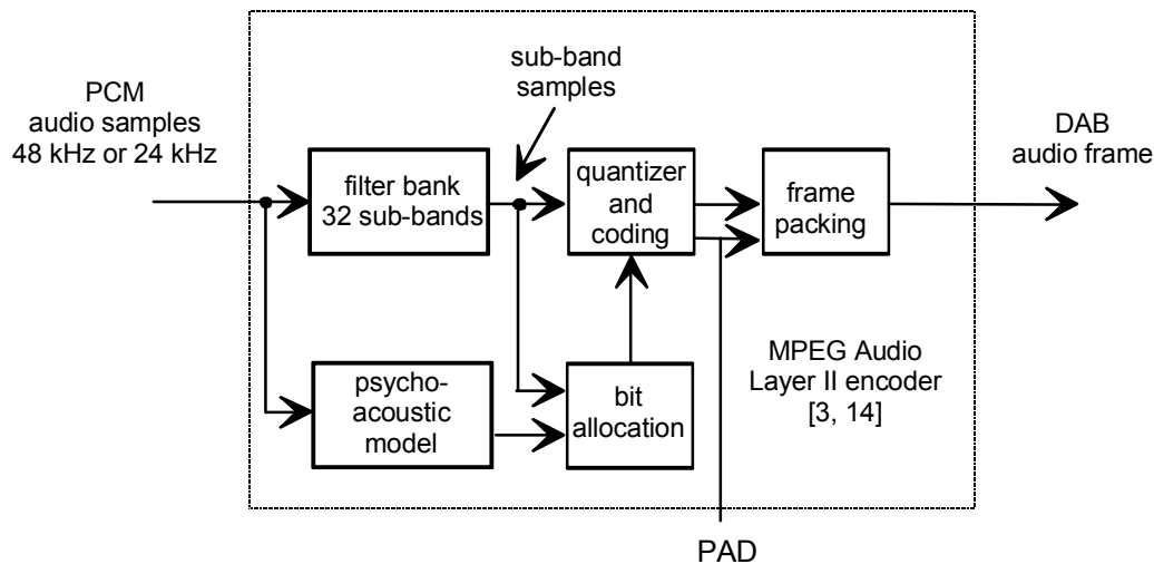
Figure 2024: Simplified block diagram of the DAB audio encoder
