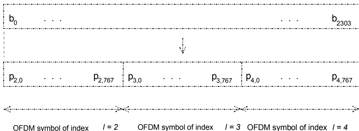
Figure 7598: Block partitioning in the FIC for transmission mode II
