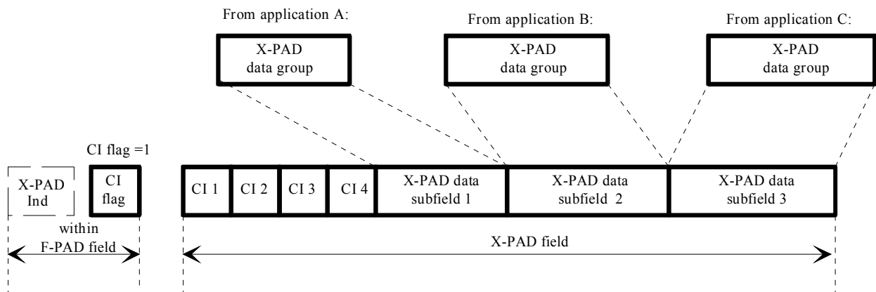
Figure 2930: Three X-PAD data groups carried in one X-PAD field
