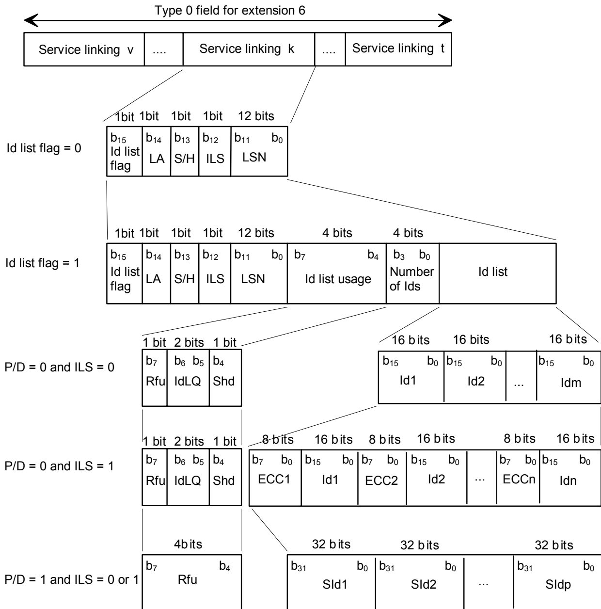
Figure 5759: Structure of the Service linking field
