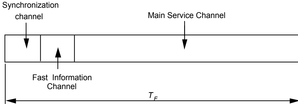
Figure 7295: Transmission frame structure
