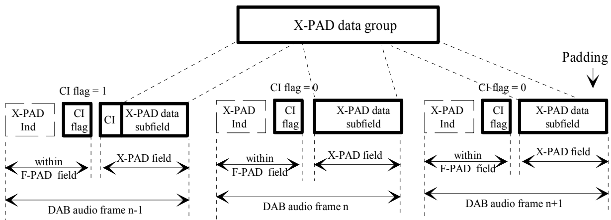
Figure 2829: An X-PAD data group extending over three consecutive X-PAD fields
