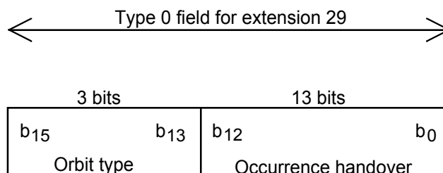
Figure 6264: Structure of the satellite handover field
