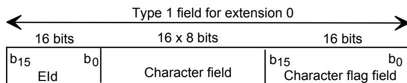
Figure 5254: Structure of the ensemble label field
