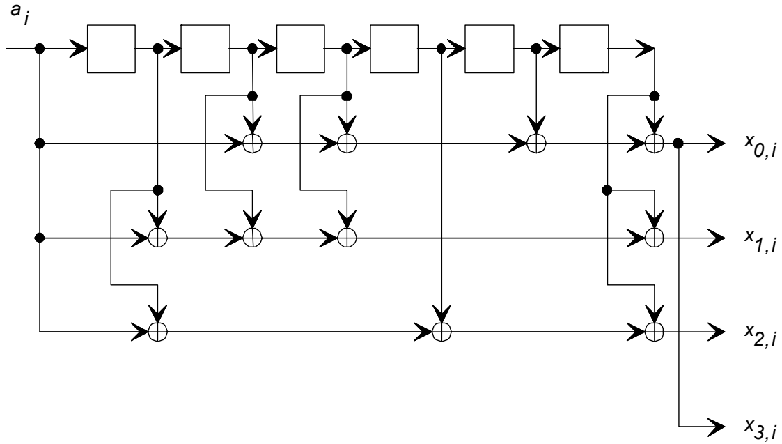
Figure 6790: Convolutional encoder
