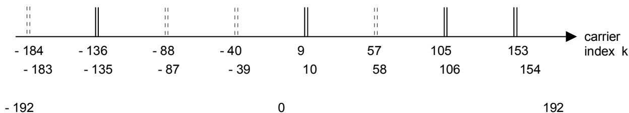
Figure 82405: Example of TII signal in transmission mode II
