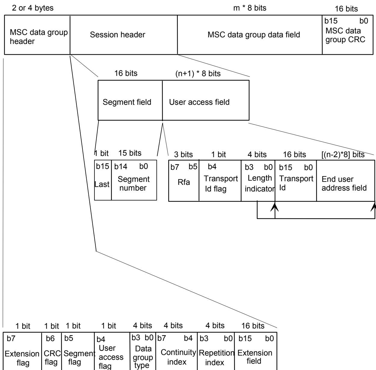
Figure 89: Structure of the MSC data group
