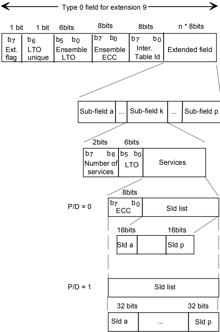
Figure 3638: Structure of the country field
