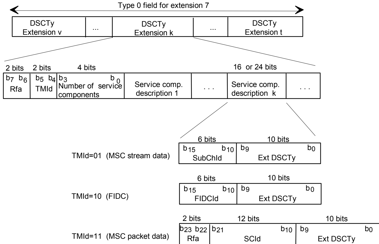
Figure 1748: Structure of the DSCTy extension field
