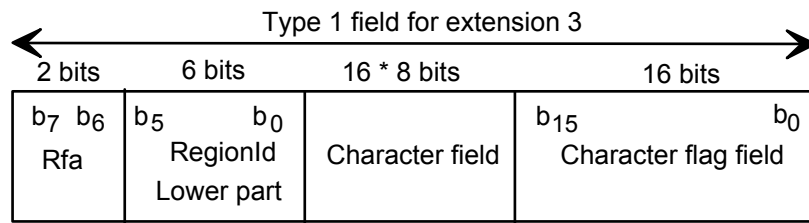
Figure 5964: Structure of the region label field
