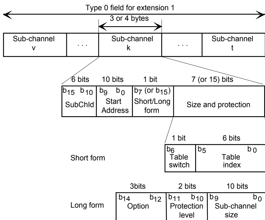
Figure 1243: Structure of the sub-channel organization field
