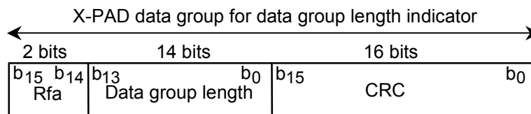
Figure 3233 : Structure of the X-PAD data group for the data group length indicator
