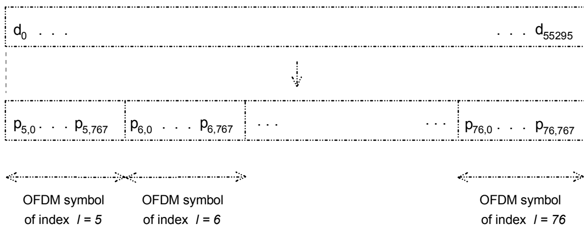
Figure 79402: Block partitioning in the MSC for transmission mode II
