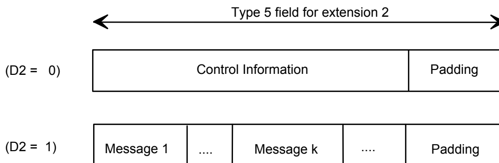
Figure 6568: Structure of Emergency Warning System field
