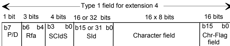
Figure 5557: Structure of the service component label field
