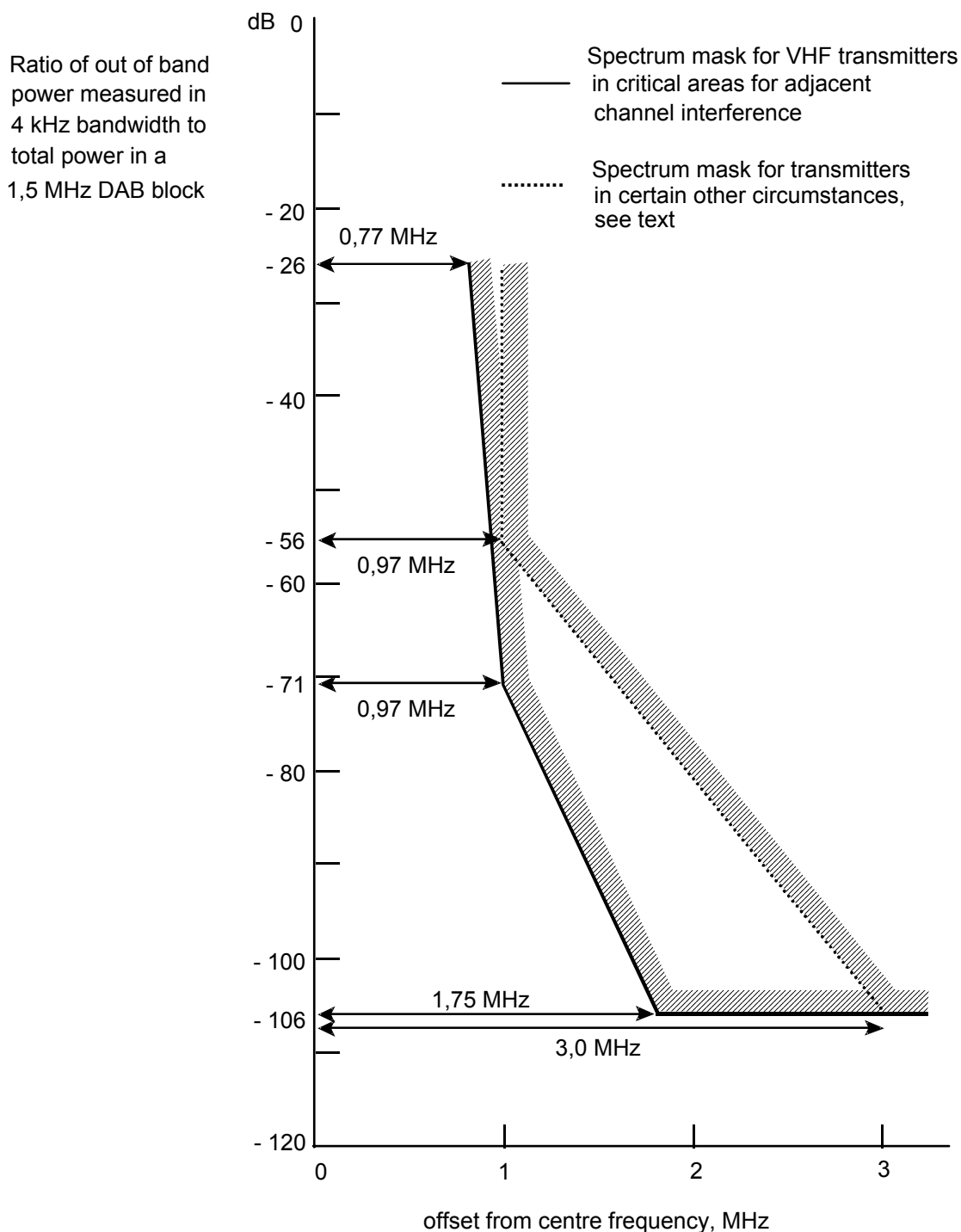
Figure 87449: Out-of-band spectrum mask for DAB transmission signal (all transmission modes)
