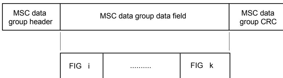
Figure 1044: MSC data group structure for carrying FIGs
