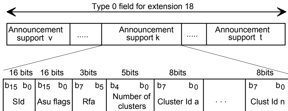
Figure 4143: Structure of announcement support field
