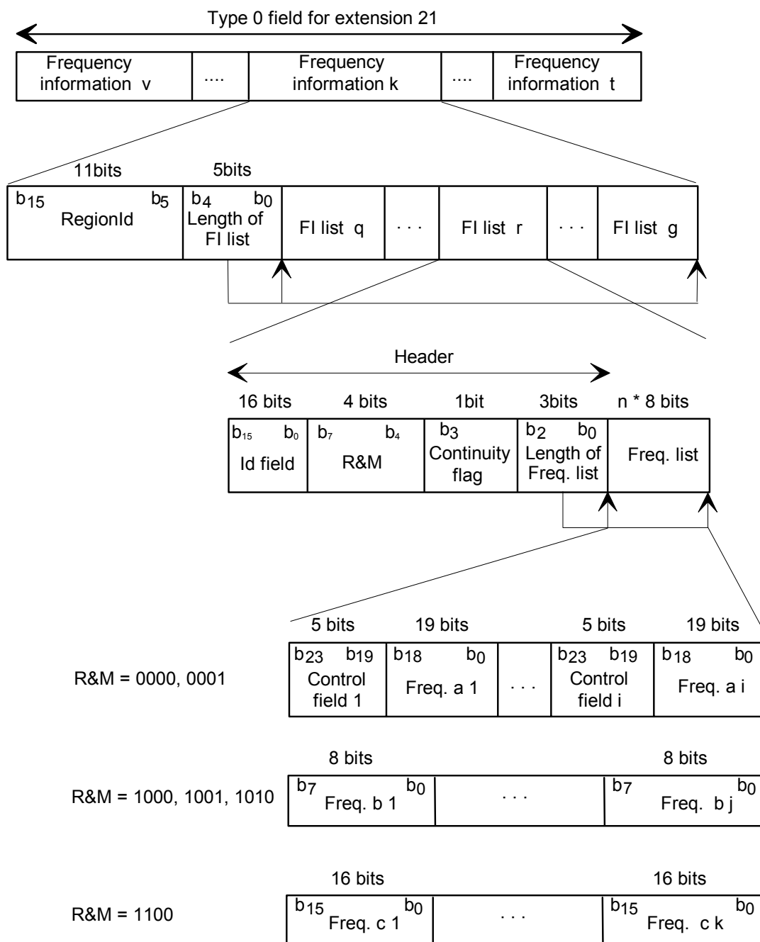
Figure 4446: Structure of the Frequency Information field
