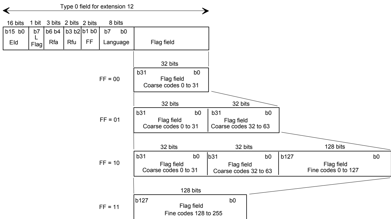
Figure 4042: Structure of the Programme Type preview field
