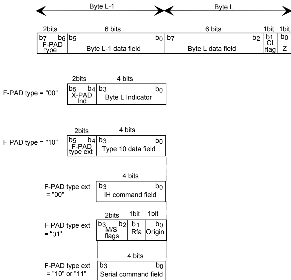
Figure 2728: Structure of the F-PAD field
