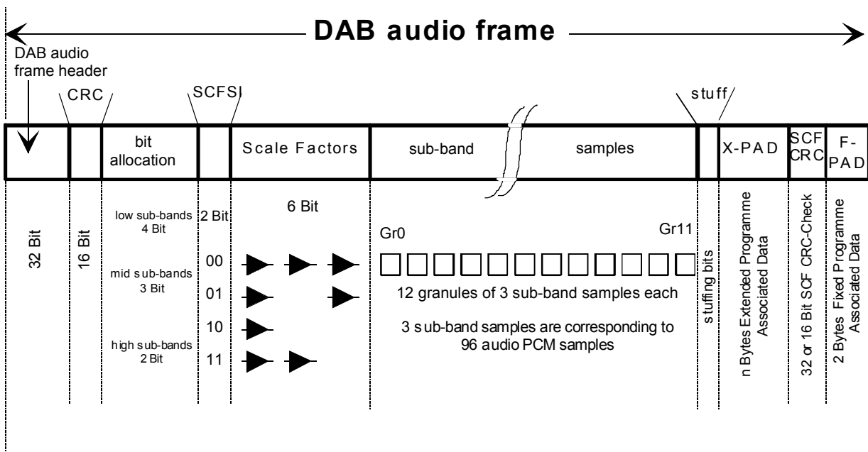
Figure 2425: Structure of the DAB audio frame
