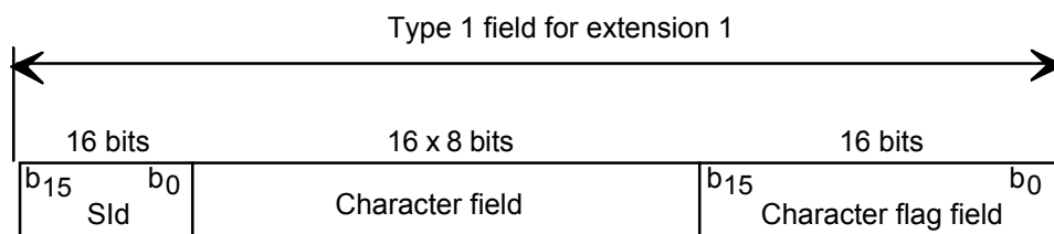
Figure 5355: Structure of the service label field
