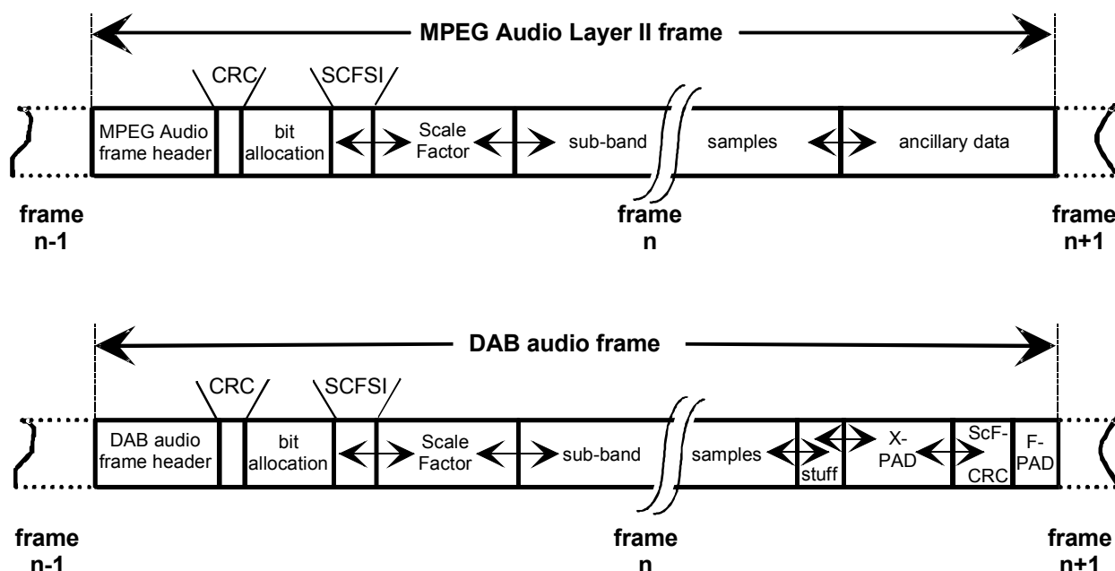
Figure 23-24: Frame structure of MPEG Audio Layer II [3, 14] and corresponding DAB audio frame
