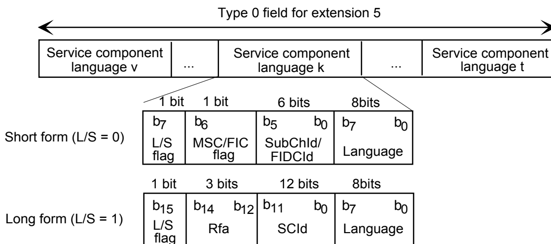
Figure 3436: Structure of the service component language field
