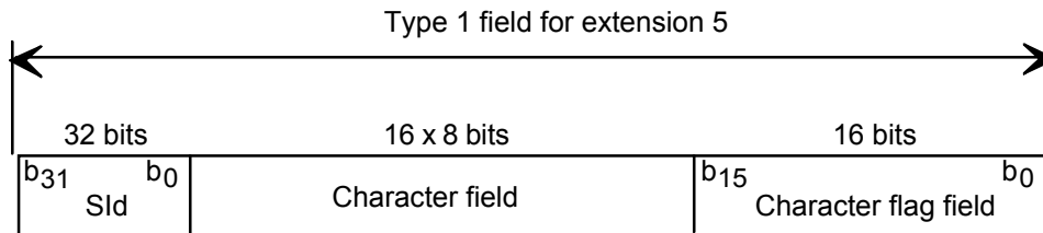
Figure 5456: Structure of the data service label field
