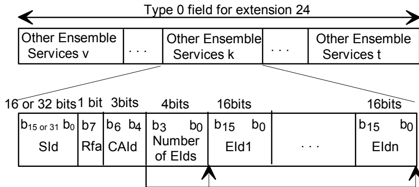
Figure 4648: Structure of the other ensembles services field
