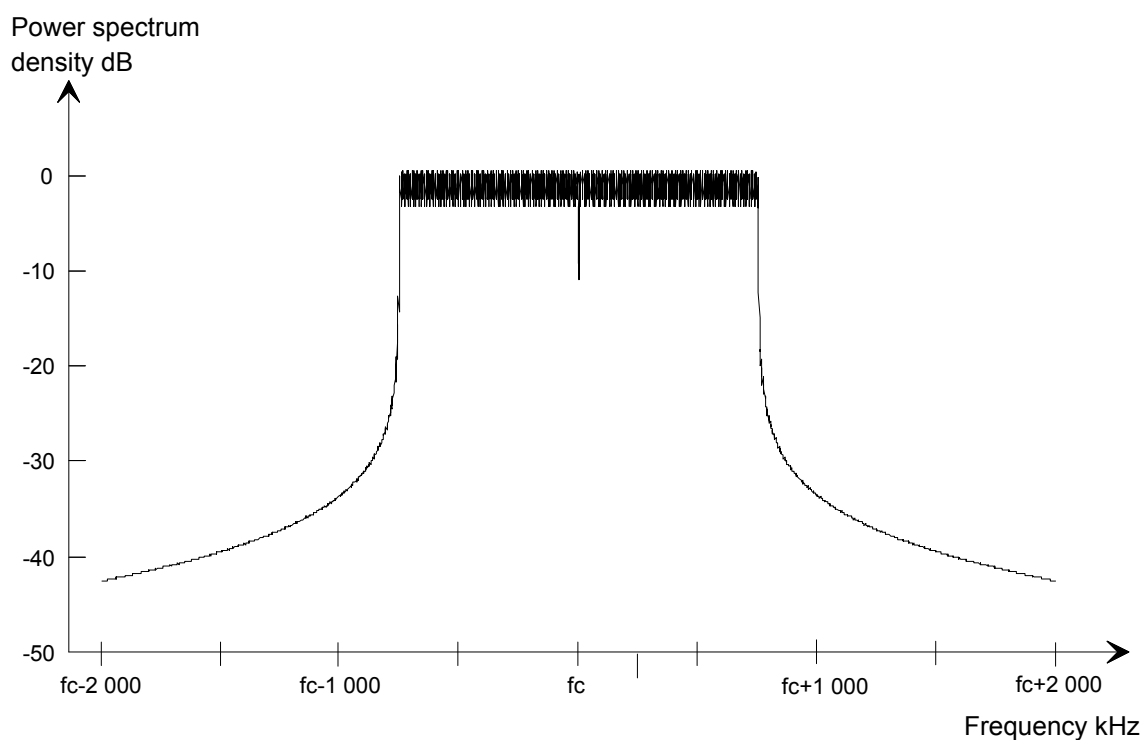
Figure 84407: Theoretical DAB transmission signal spectrum for transmission mode II
