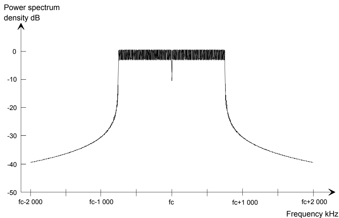
Figure 85408: Theoretical DAB transmission signal spectrum for transmission mode III
