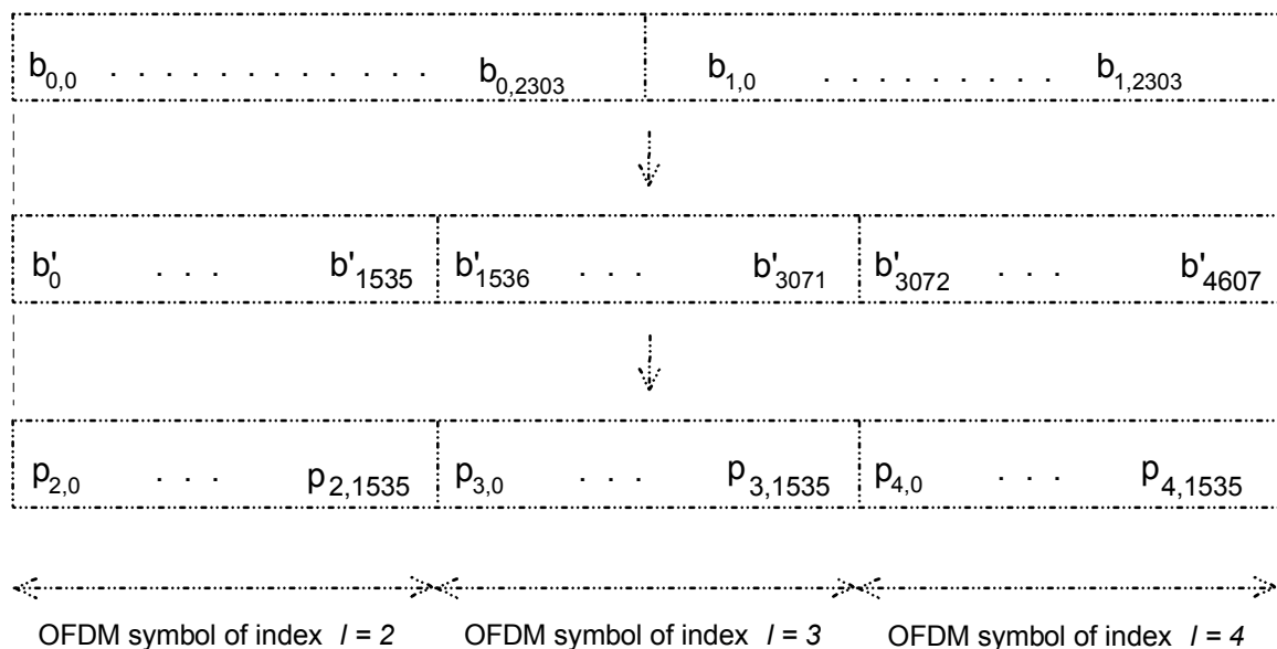
Figure 77400: Block partitioning in the FIC for transmission mode IV
