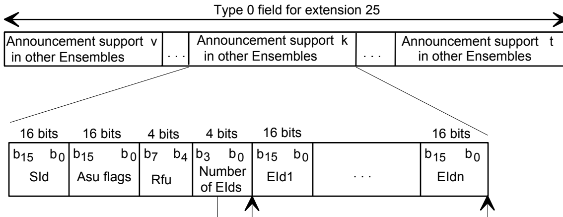
Figure 4749: Structure of other ensembles announcement support field
