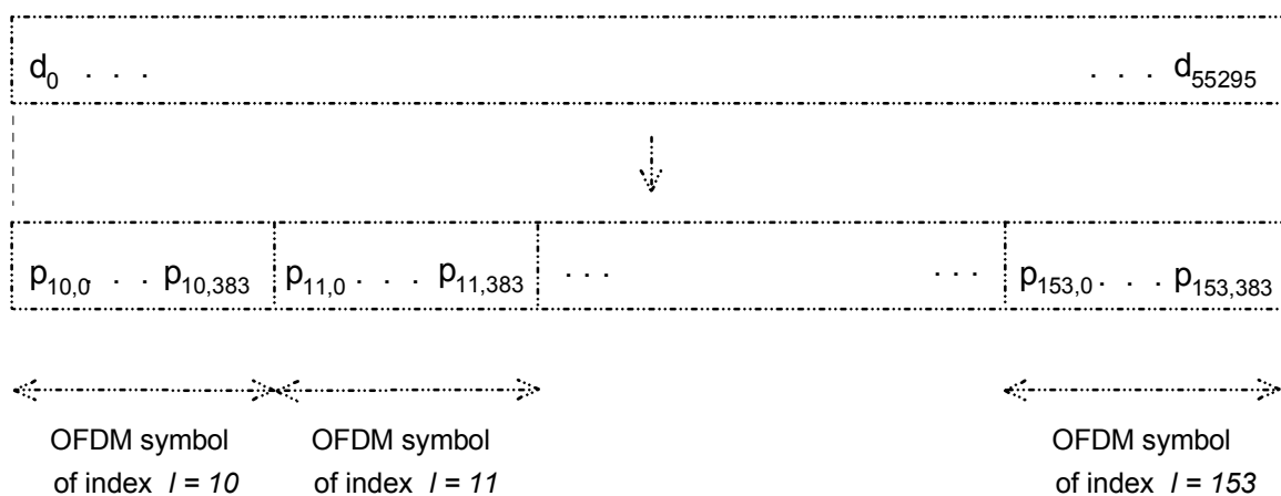
Figure 80403: Block partitioning in the MSC for transmission mode III
