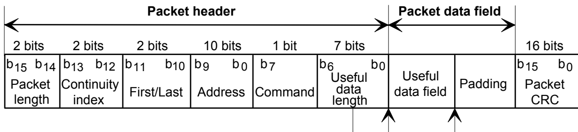
Figure 78: Packet structure
