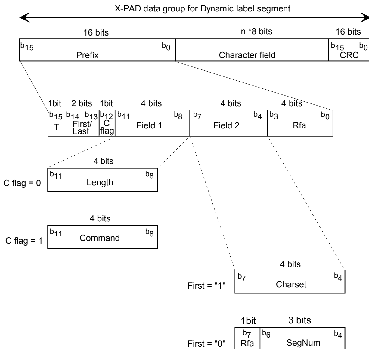
Figure 3335: Structure of the X-PAD data group for each dynamic label segment
