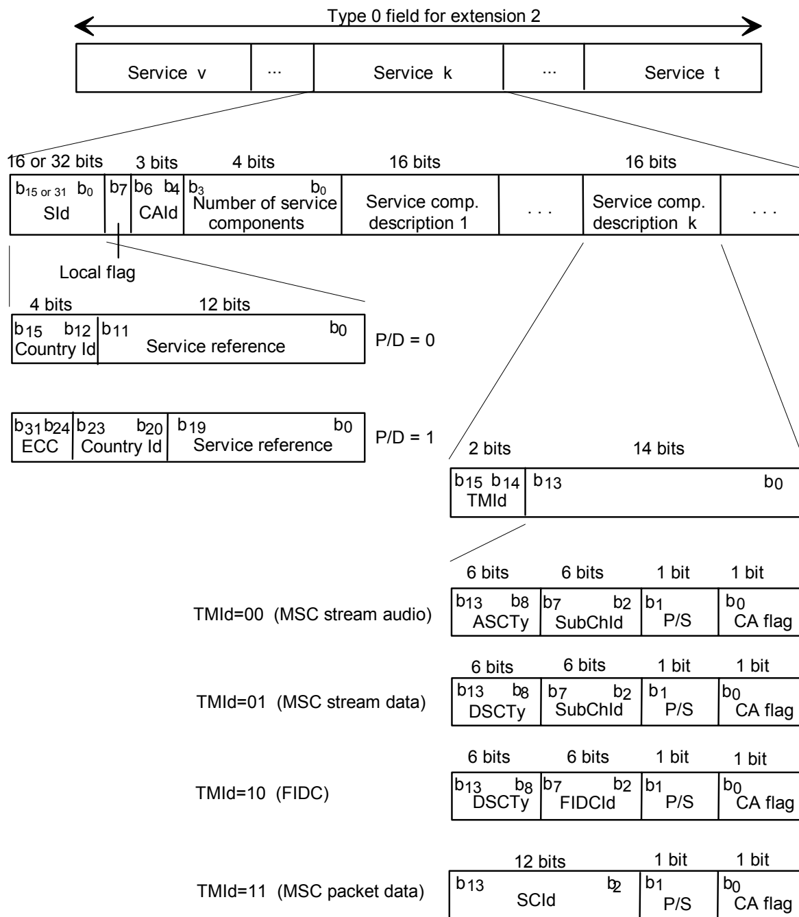
Figure 1344: Structure of the service organization field
