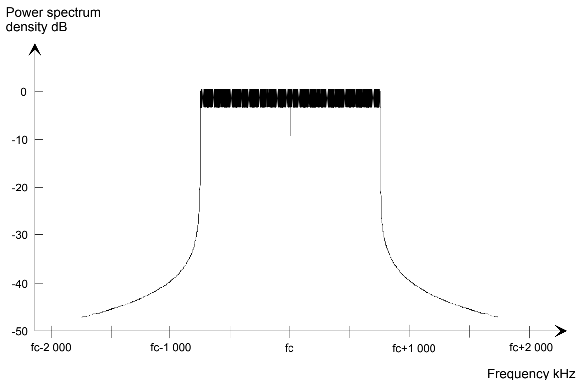
Figure 83406: Theoretical DAB transmission signal spectrum for transmission mode I
