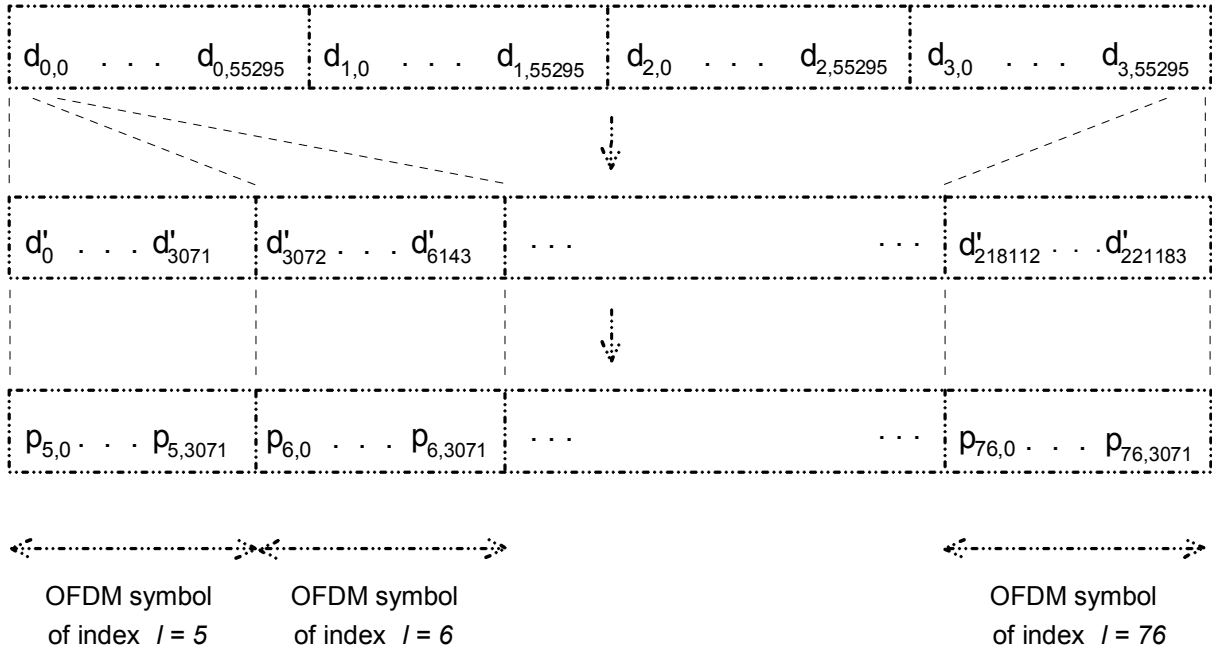
Figure 78101 : Block partitioning in the MSC for transmission mode I
