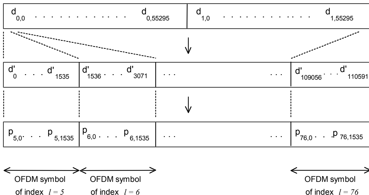
Figure 81404: Block partitioning in the MSC for transmission mode IV
