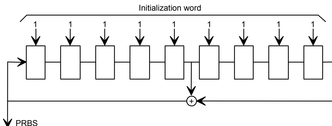
Figure 6689: PRBS generator
