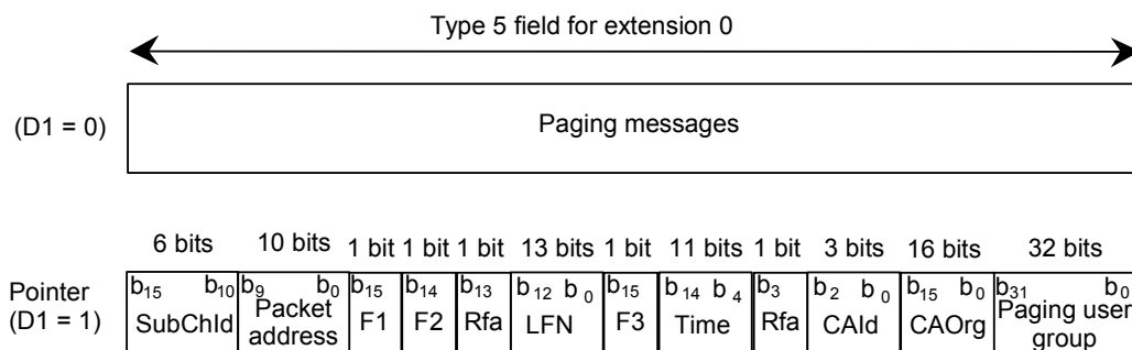
Figure 6466: Structure of the paging field
