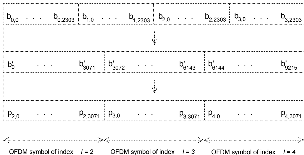
Figure 7497: Block partitioning in the FIC for transmission mode I
