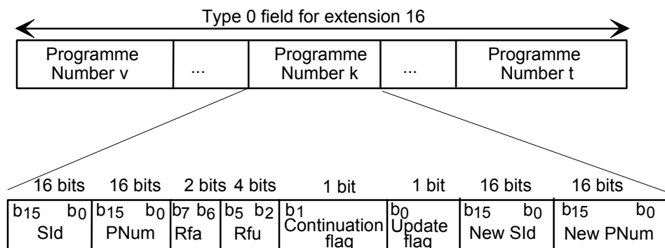
Figure 3739: Structure of Programme Number field
