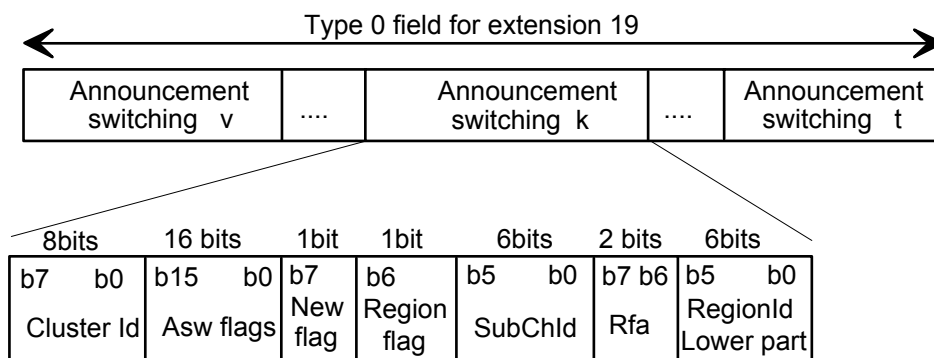
Figure 4244: Structure of announcement switching field
