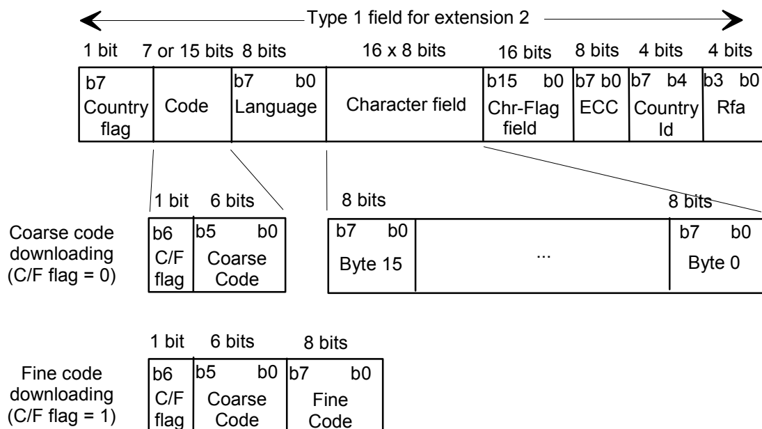
Figure 3941: Structure of the Programme Type downloading field
