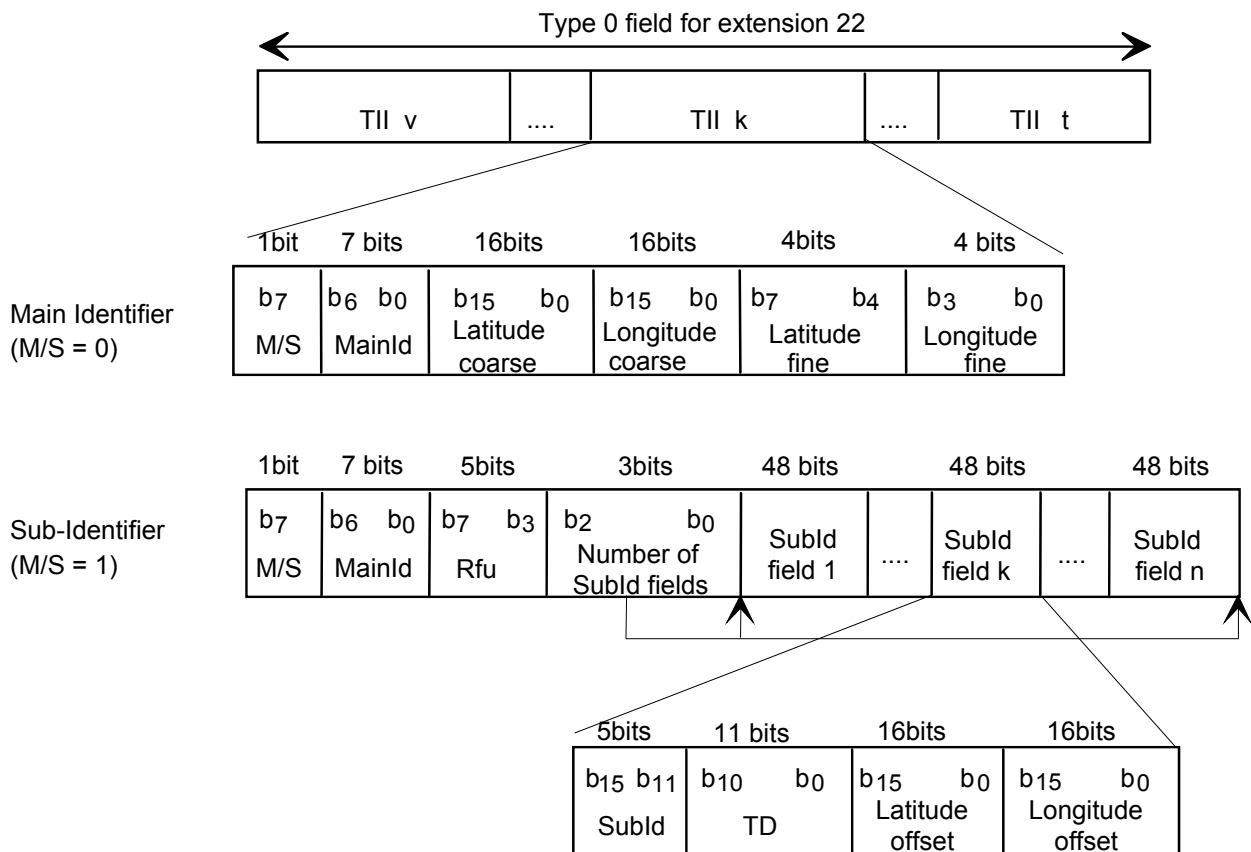
Figure 4547: Structure of the Transmitter Identification Information (TII) field
