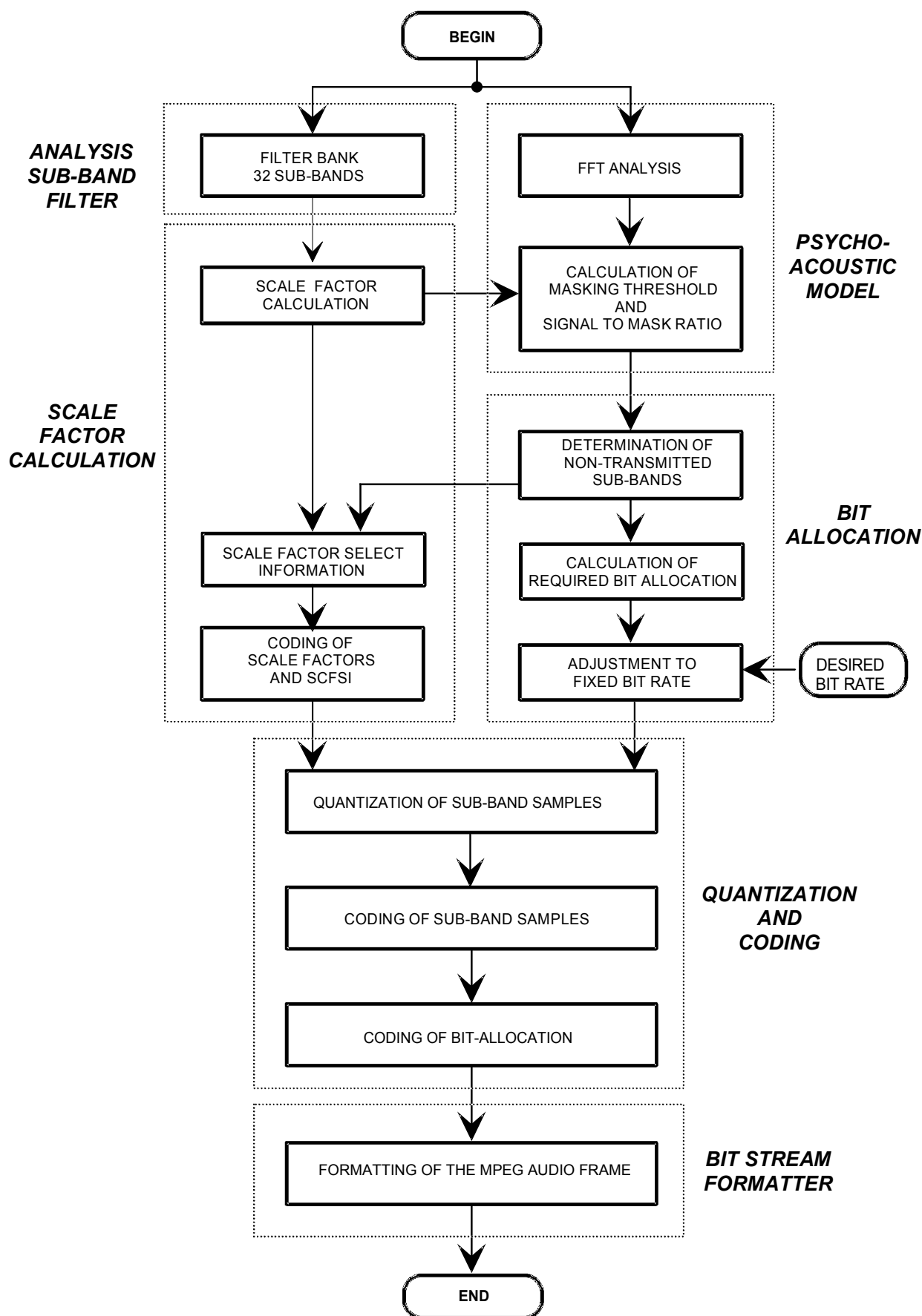
Figure 2223: Flow diagram of the MPEG Audio Layer II [3, 14] encoder
