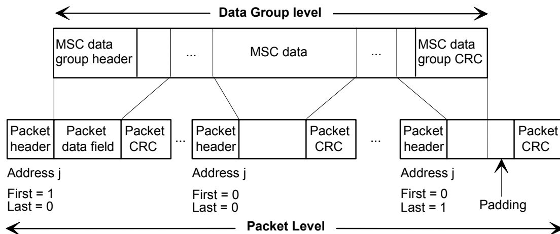
Figure 940: Relationship between a MSC data group and a sequence of packets
