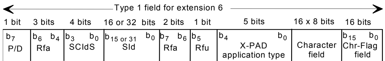
Figure 5658: Structure of the X-PAD user application label field
