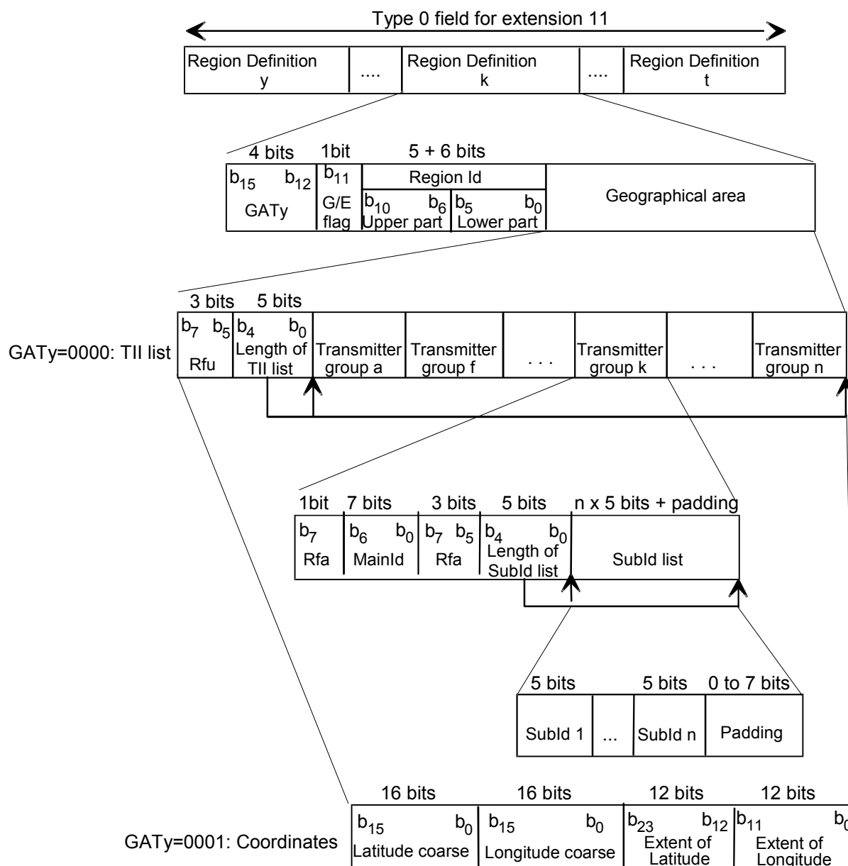
Figure 5860: Structure of regional definition information
