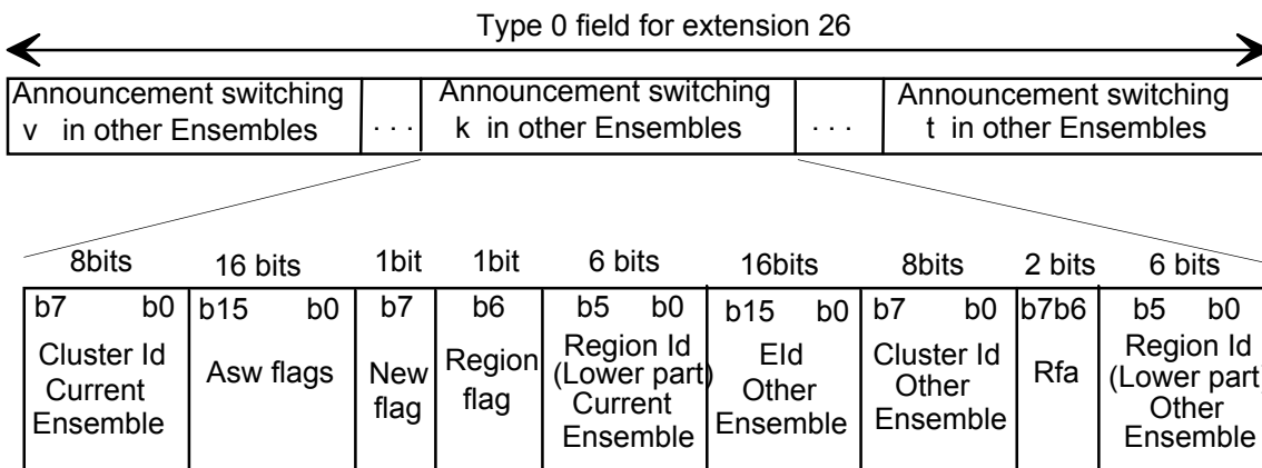
Figure 4850: Structure of announcement switching field
