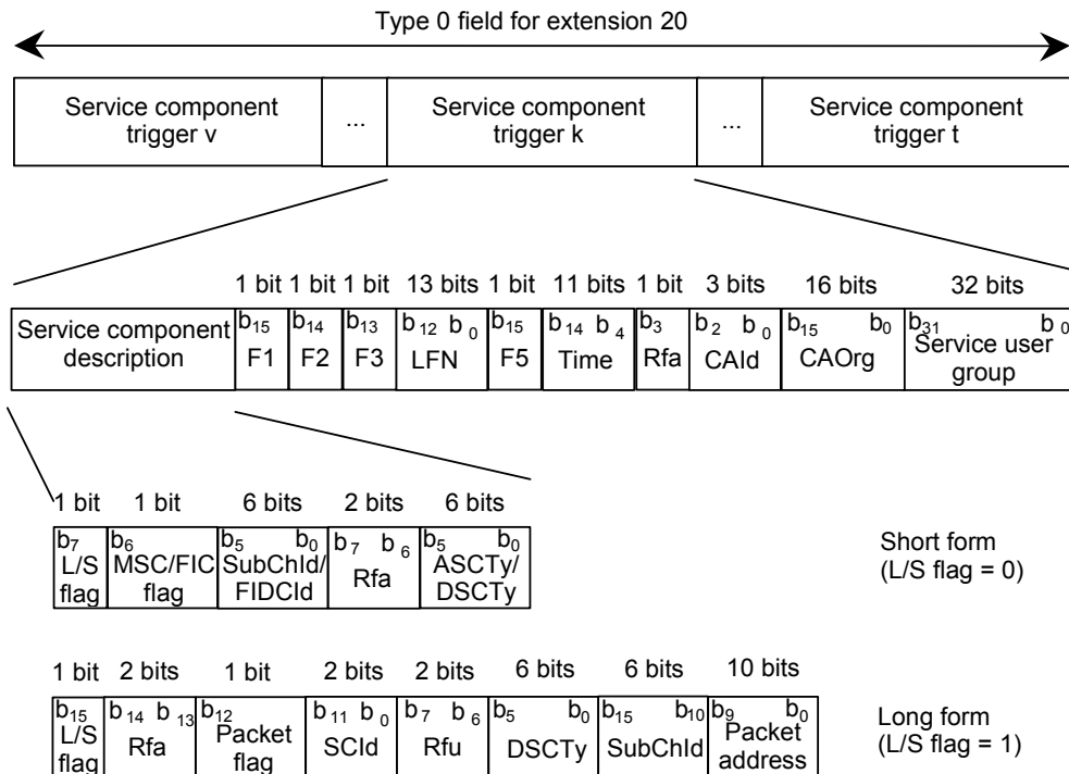
Figure 4345: Structure of the service component trigger field
