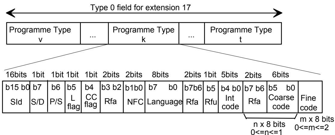
Figure 3840: Structure of the Programme Type field
