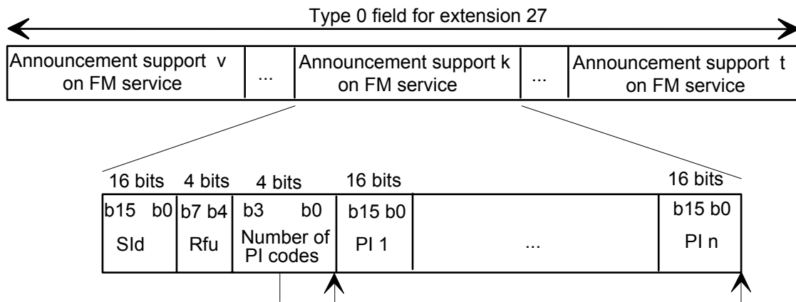
Figure 4954: Structure of the FM services announcement support field
