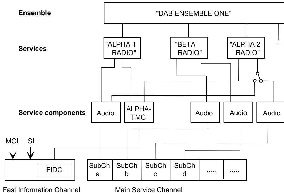
Figure 1142: An example of the DAB service structure
