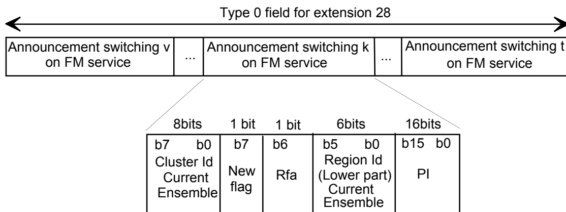
Figure 5052: Structure of the FM services announcement switching field
