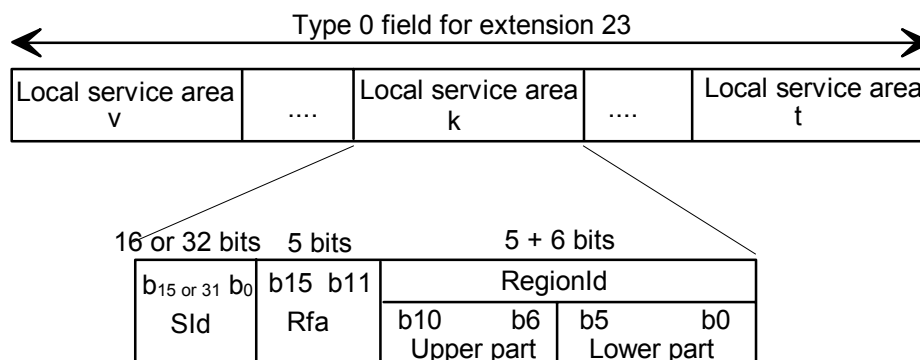
Figure 6062: Structure of Local service area field
